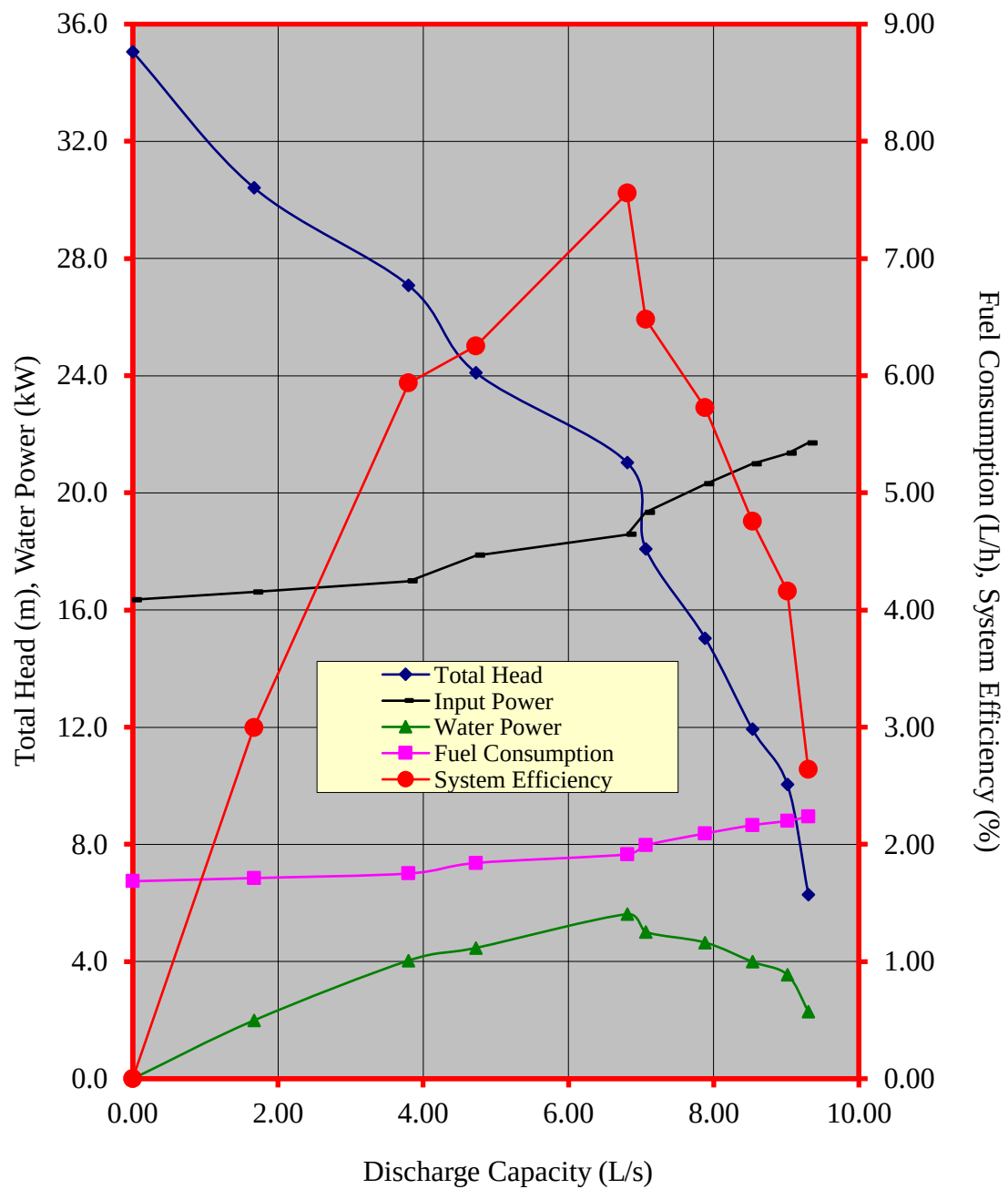
Figure 3. Performance characteristic curves of the PLATINUM PT5.5 HP self-priming centrifugal pumpset
